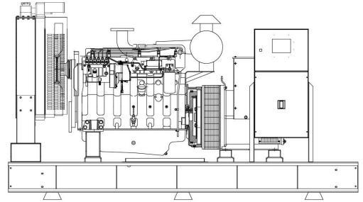
WITHOUT CANOPY
