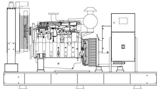
WITHOUT CANOPY
