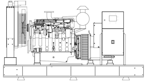
WITHOUT CANOPY
