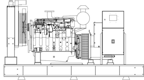
WITHOUT CANOPY
