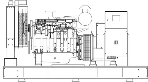
WITHOUT CANOPY
