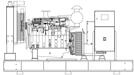
WITHOUT CANOPY
