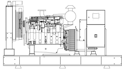
WITHOUT CANOPY
